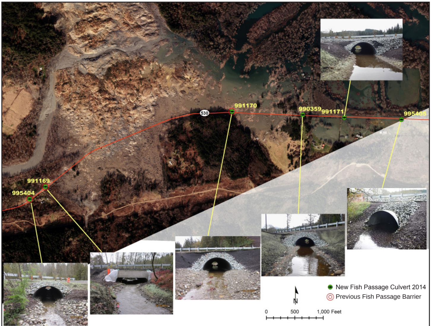
Figure 3. Landslide impacts to SR 530 requiring 6 new culvert crossings
